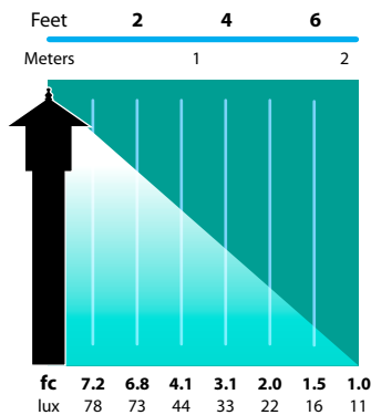
AL-10 Half Spread Photometrics 14 ft. (4.3m) diameter 24" above grade
