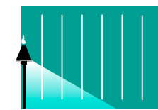
AL-18-SM Half Spread Photometrics 12ft (3.7m) diameter
