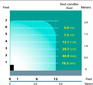
DL-41-VERT Half Spread Photometrics
