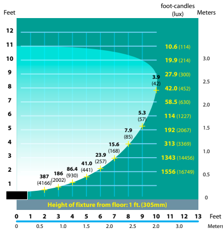
FFL-78 Half Spread Photometrics
