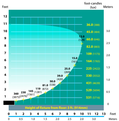
FFL-52 Half Spread Photometrics
