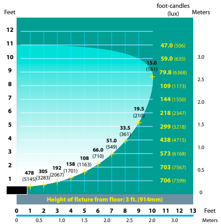
FFL-78 Half Spread Photometrics
