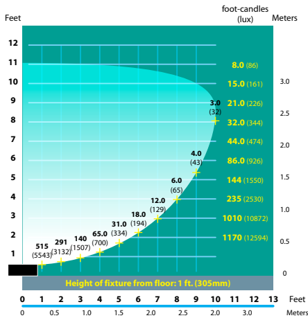
FFL-52 Half Spread Photometrics
