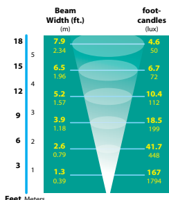
18w PAR36 (QWFL) Vertical 25° angle beam
