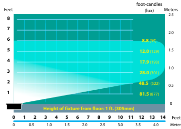
SL-08-AL-FL-7 Half Spread Photometrics (7w)
