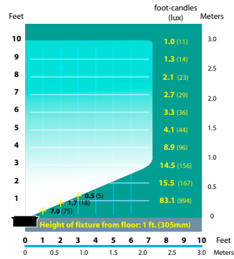
SL-08 Half Spread Photometrics
