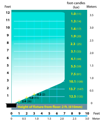
SL-08-AL Half Spread Photometrics
