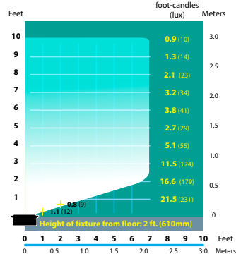
SL-08 Half Spread Photometrics
