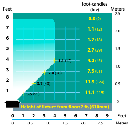
SL-31 Half Spread Photometrics
