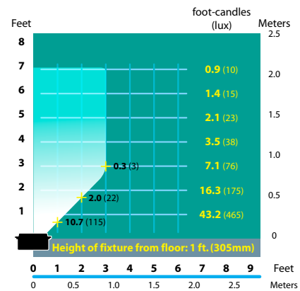
SL-31 Half Spread Photometrics
