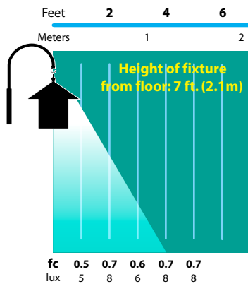
SL-13 Half Spread Photometrics 4 ft. (1.2m) radius
